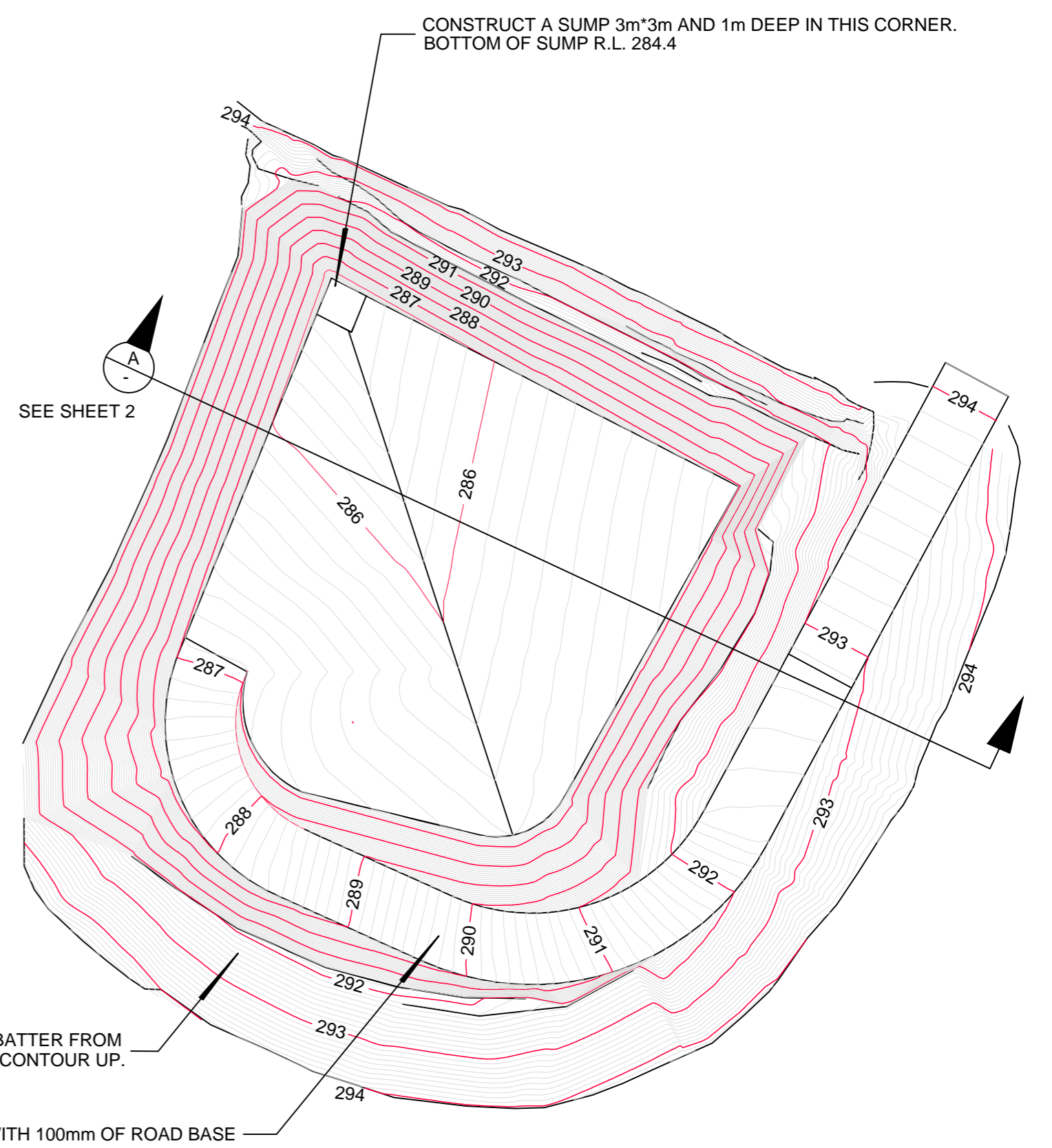
DESIGN SURFACE REDUCTION RATIO 1:400
