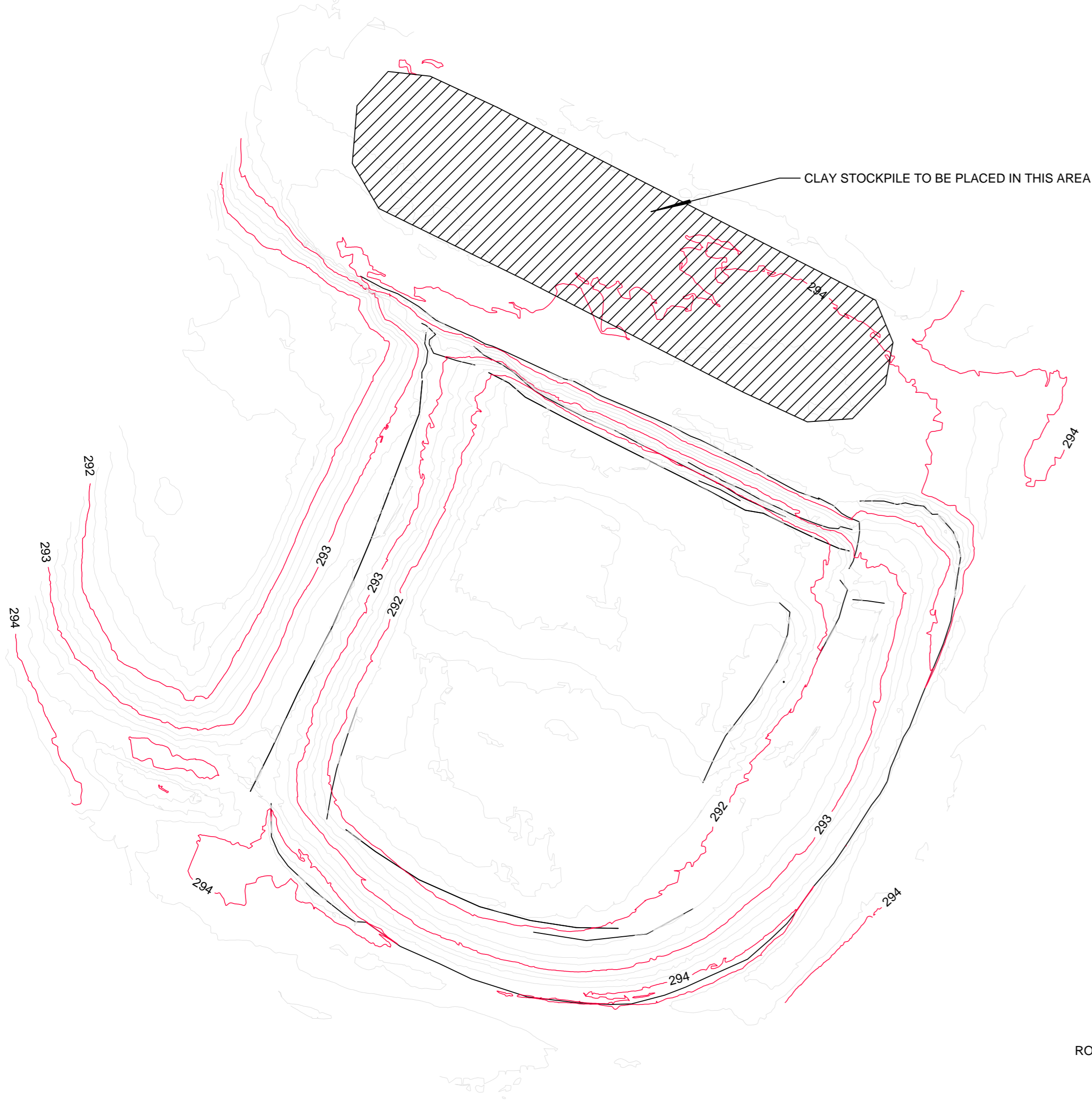
CURRENT SURFACE REDUCTION RATIO 1:400
